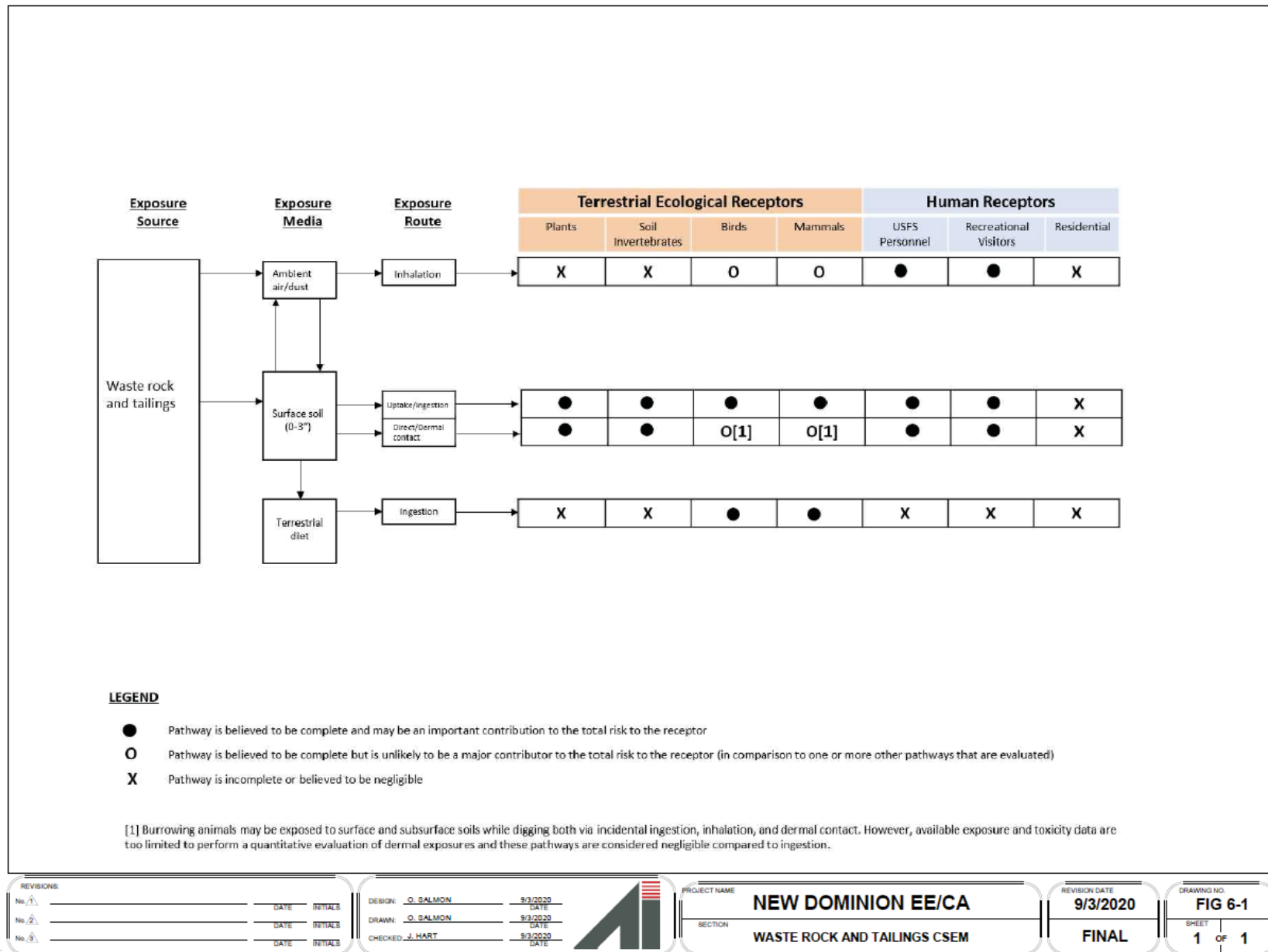
Figure 6-1. Waste Rock and Tailings Conceptual Site Exposure Model
